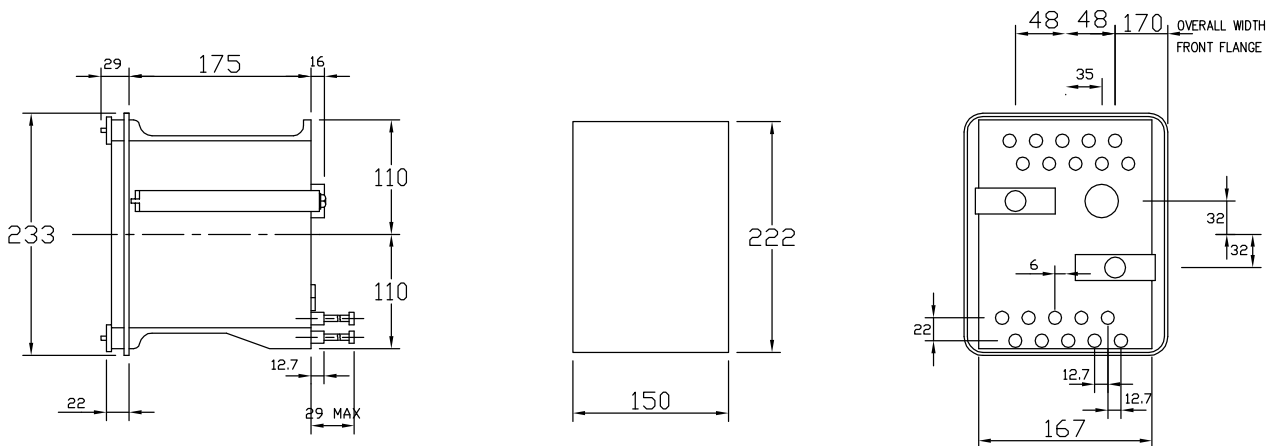
Figure 1 : Case and panel cut-out dimensions for case 1D (all dimensions in mm)
