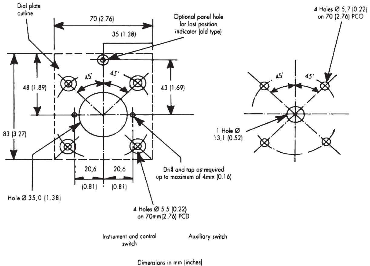
Figure 2 : Panel Drilling Details
