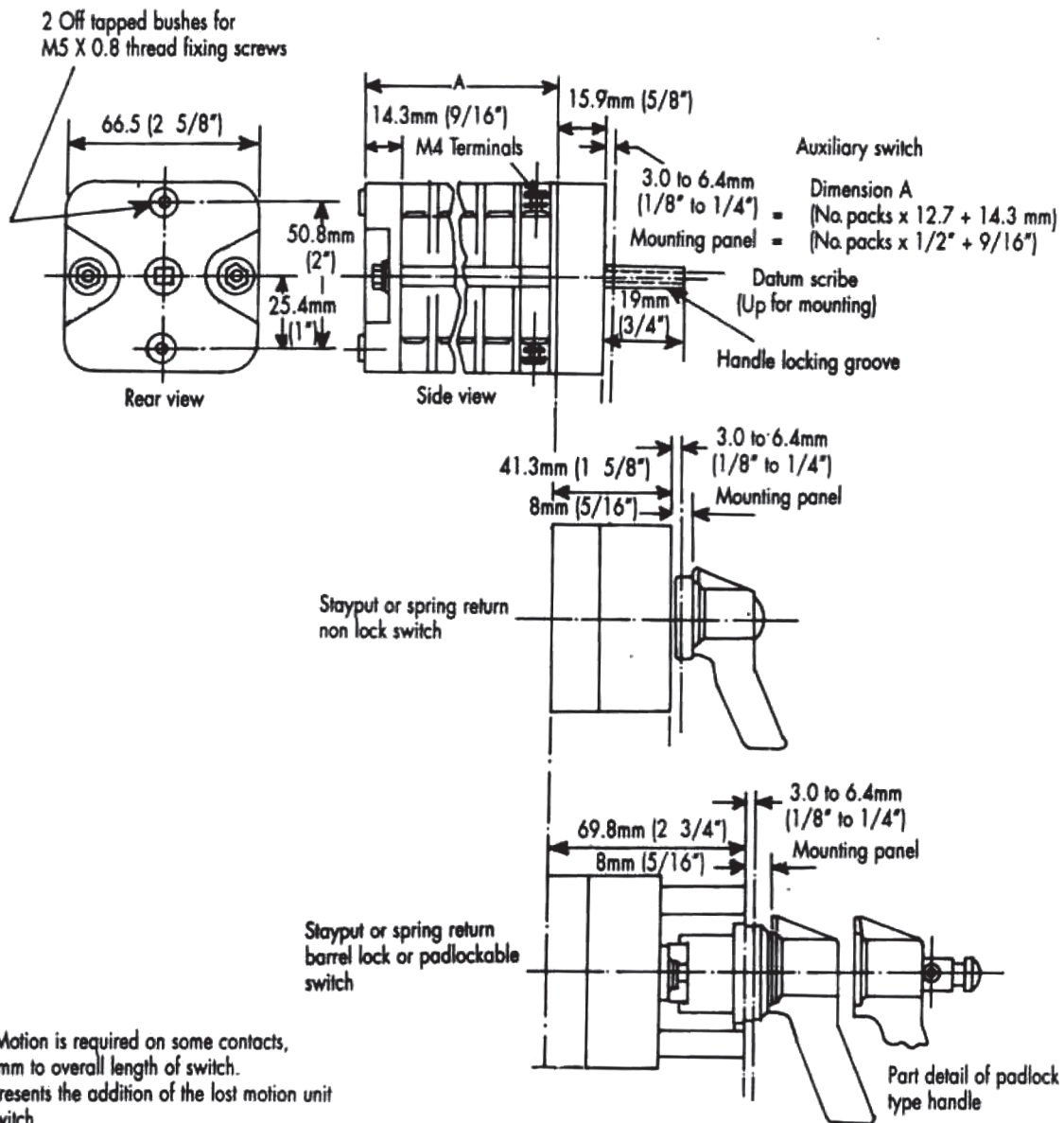
Figure 1 :Outline Dimensions
